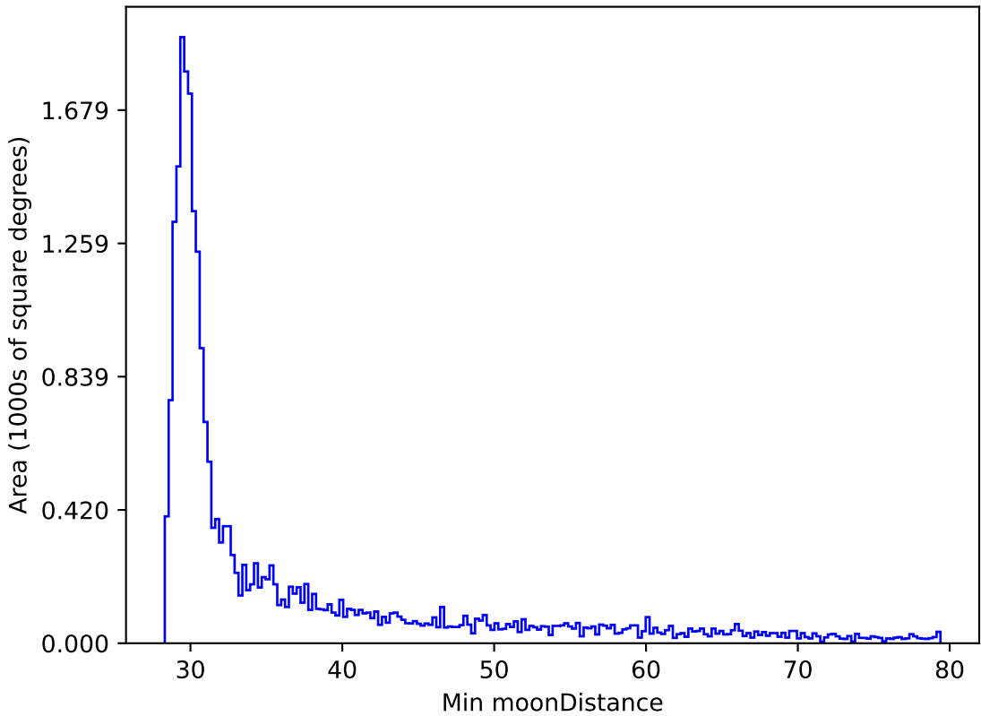
noroll_mjdp60_v3.4_10yrs All sky z band: Min moonDistance
