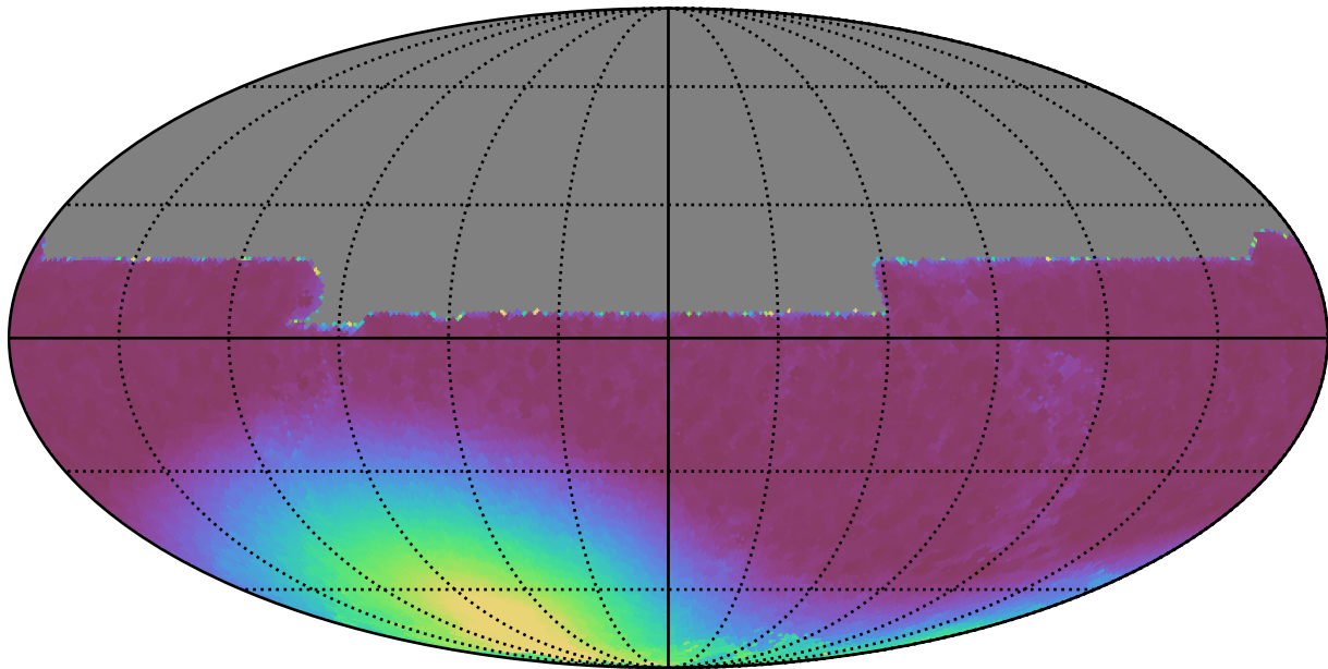
noroll_mjdp60_v3.4_10yrs All sky y band: Min moonDistance
