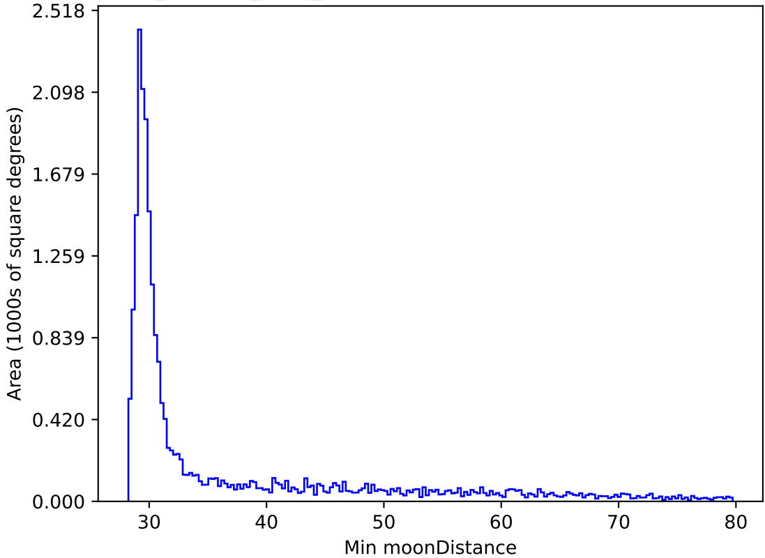
noroll_mjdp60_v3.4_10yrs All sky y band: Min moonDistance
