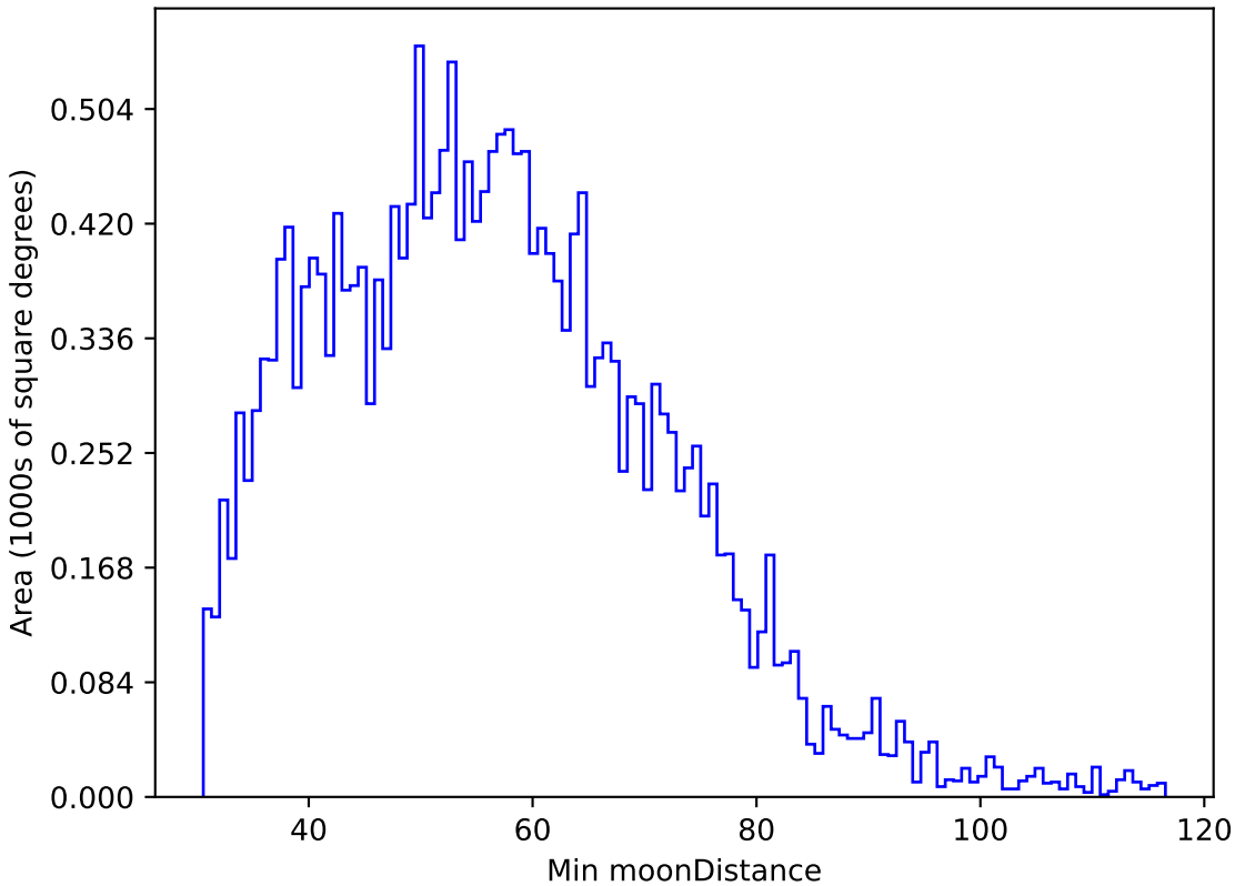
noroll_mjdp60_v3.4_10yrs All sky u band: Min moonDistance
