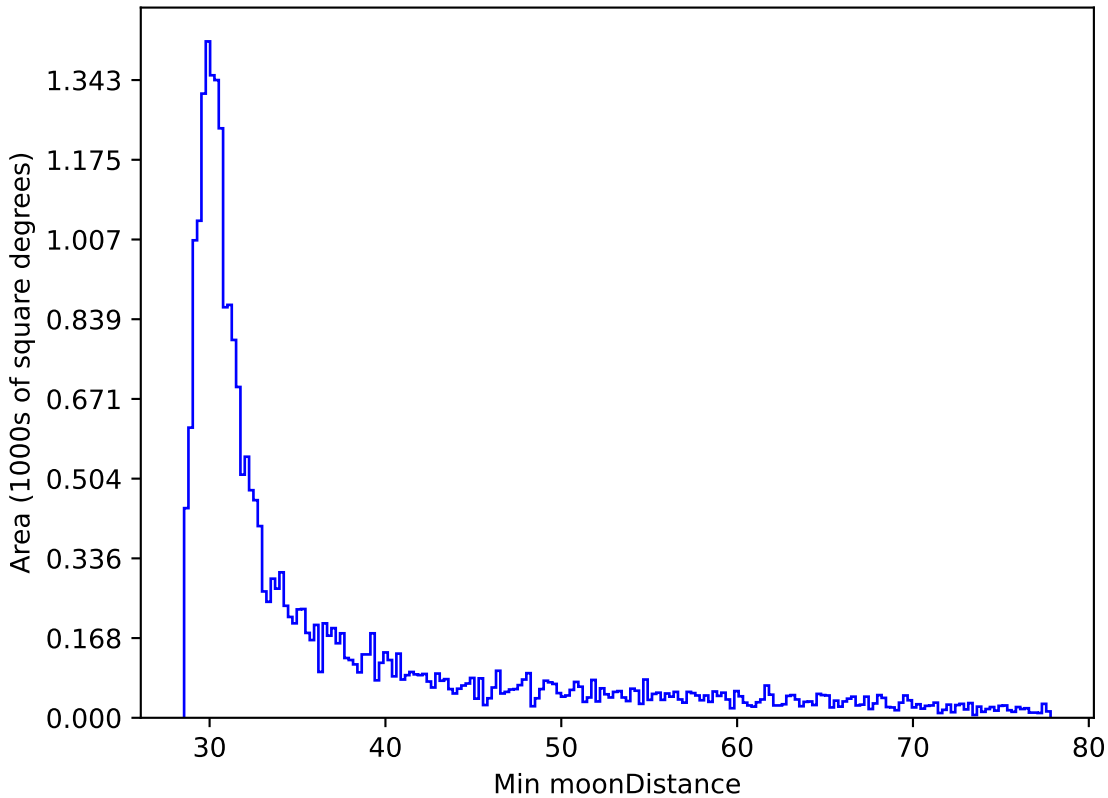
noroll_mjdp60_v3.4_10yrs All sky i band: Min moonDistance
