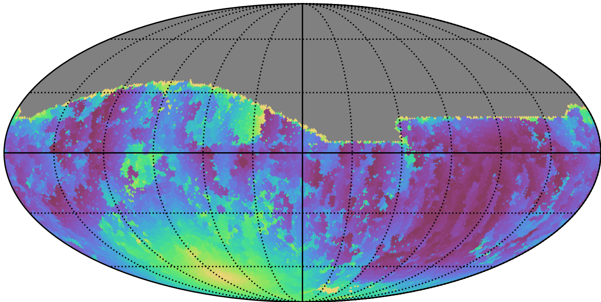
noroll_mjdp60_v3.4_10yrs All sky g band: Min moonDistance
