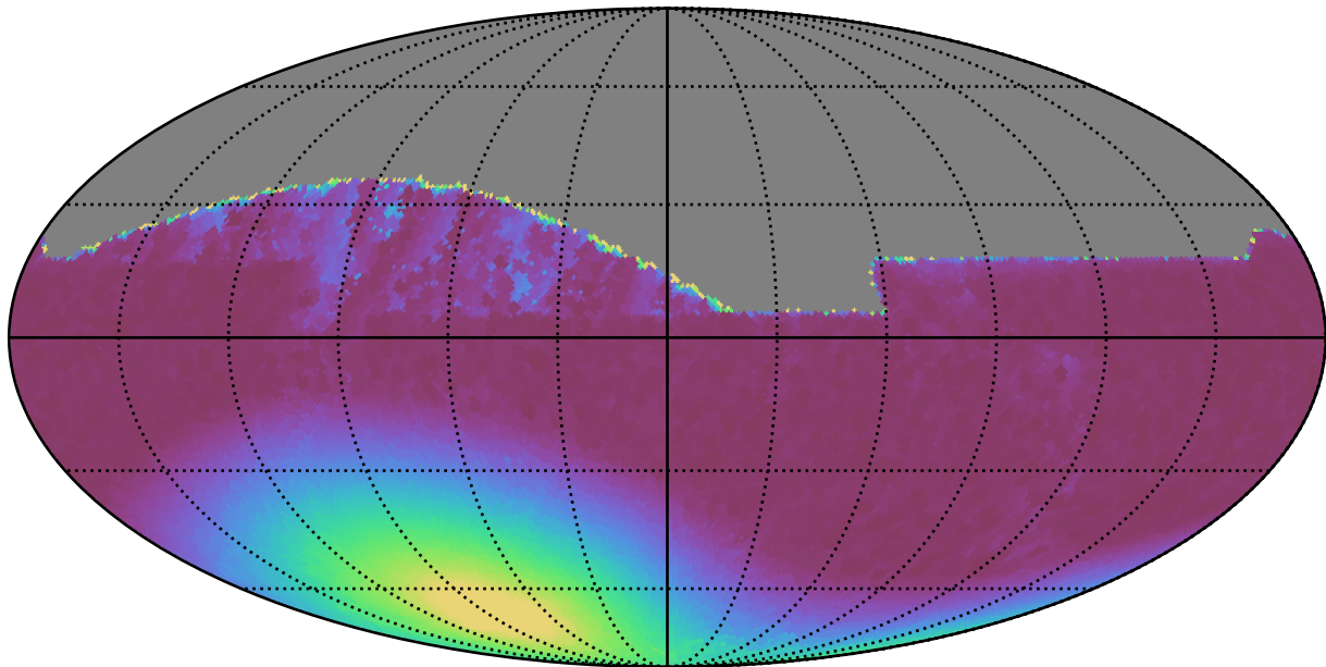
noroll_mjdp60_v3.4_10yrs All sky all bands: Min moonDistance
