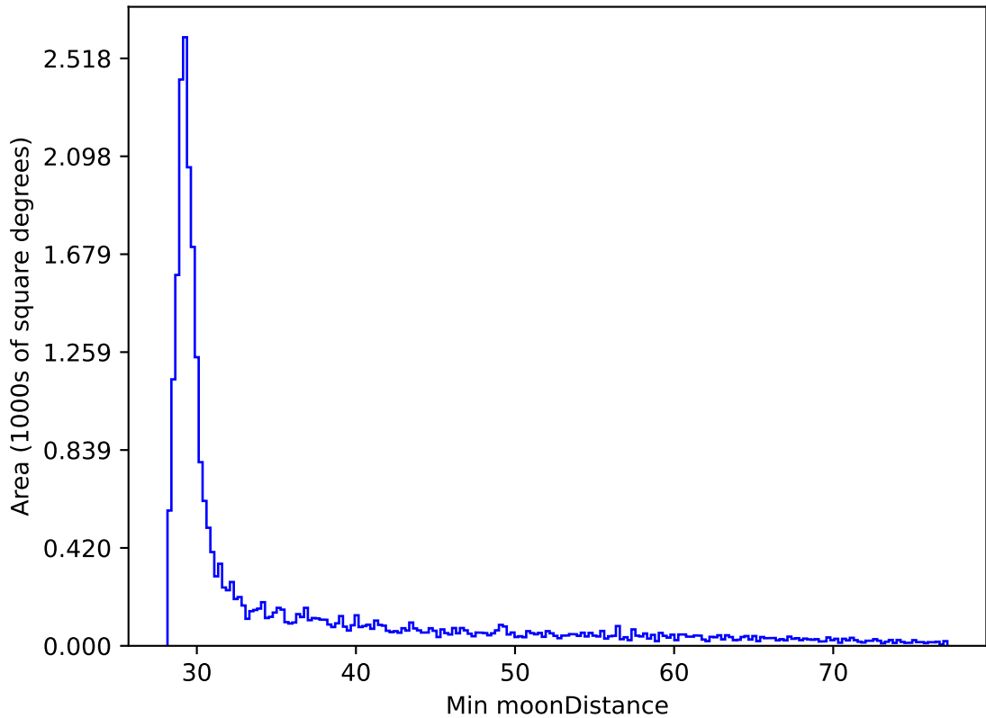
noroll_mjdp60_v3.4_10yrs All sky all bands: Min moonDistance
