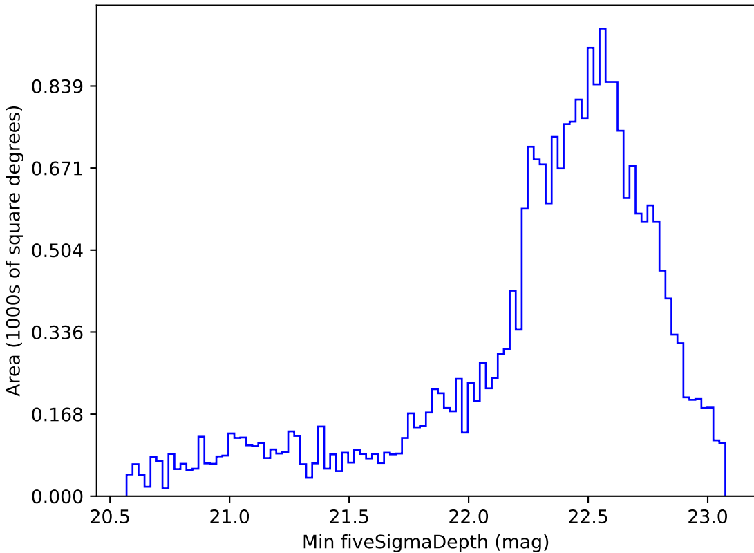
noroll_mjdp60_v3.4_10yrs Yr 1 z band: Min fiveSigmaDepth
