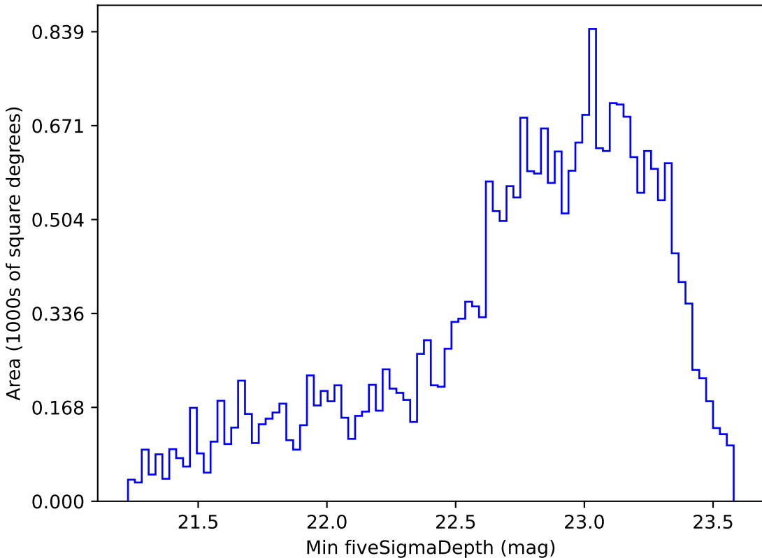
noroll_mjdp60_v3.4_10yrs Yr 1 i band: Min fiveSigmaDepth
