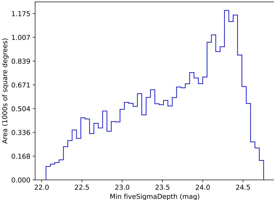
noroll_mjdp60_v3.4_10yrs Yr 1 g band: Min fiveSigmaDepth
