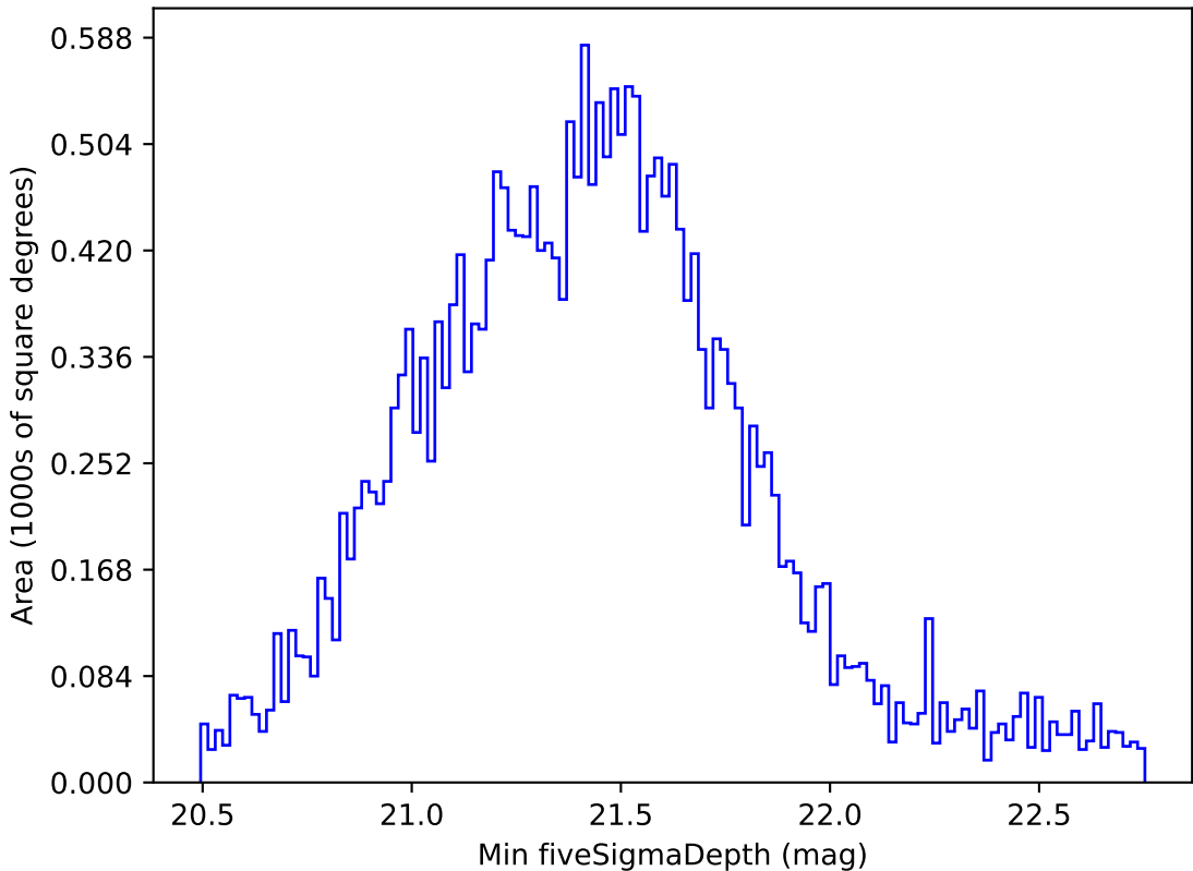
noroll_mjdp60_v3.4_10yrs Yr 1 all bands: Min fiveSigmaDepth
