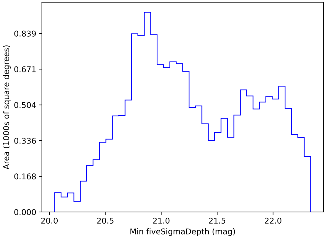
noroll_mjdp60_v3.4_10yrs WFD z band: Min fiveSigmaDepth
