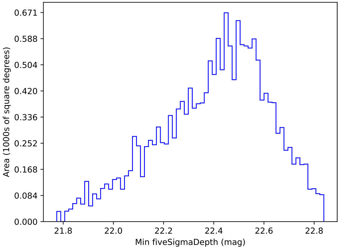
noroll_mjdp60_v3.4_10yrs WFD u band: Min fiveSigmaDepth
