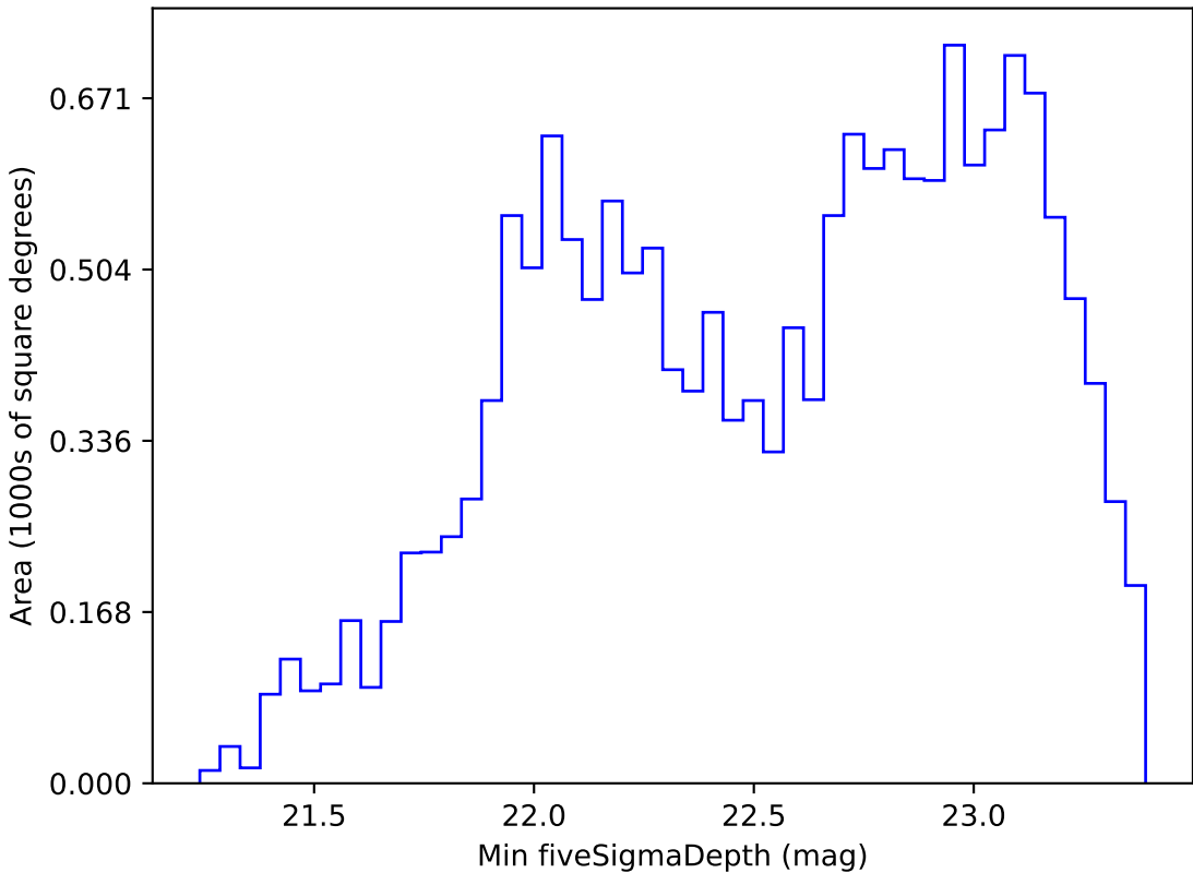
noroll_mjdp60_v3.4_10yrs WFD r band: Min fiveSigmaDepth
