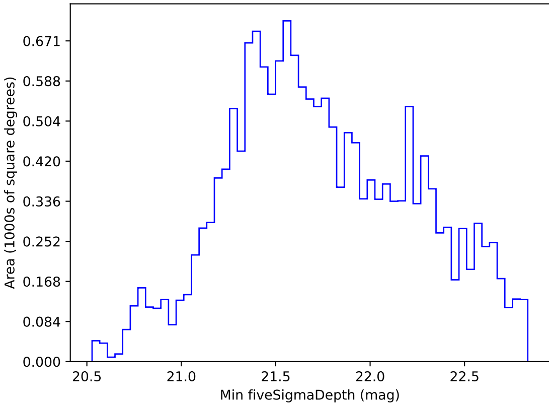
noroll_mjdp60_v3.4_10yrs WFD i band: Min fiveSigmaDepth
