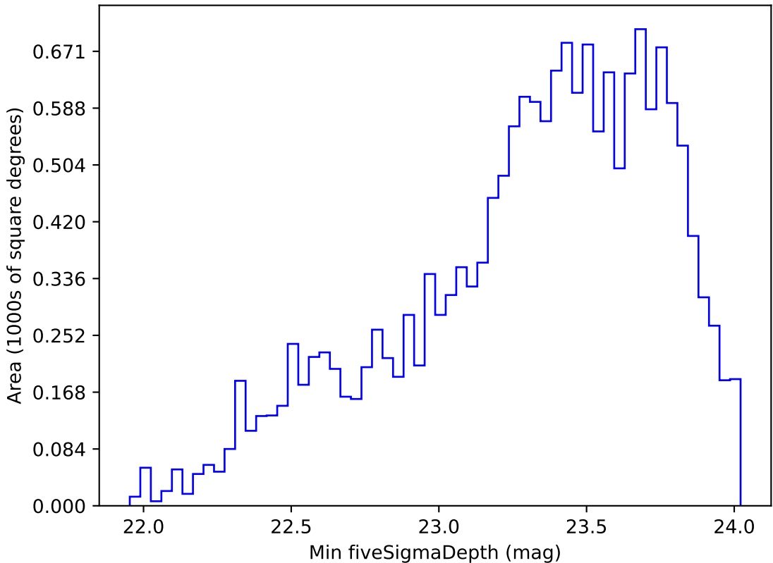
noroll_mjdp60_v3.4_10yrs WFD g band: Min fiveSigmaDepth
