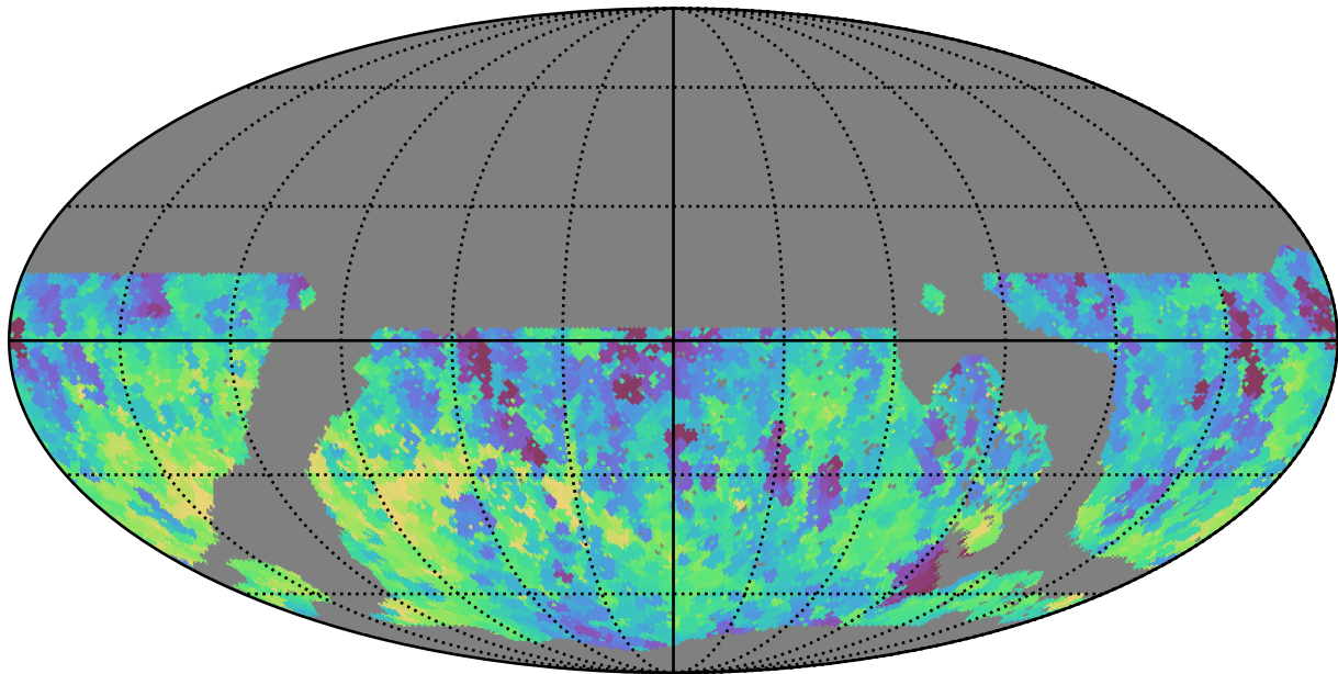
noroll_mjdp60_v3.4_10yrs WFD all bands: Min fiveSigmaDepth
