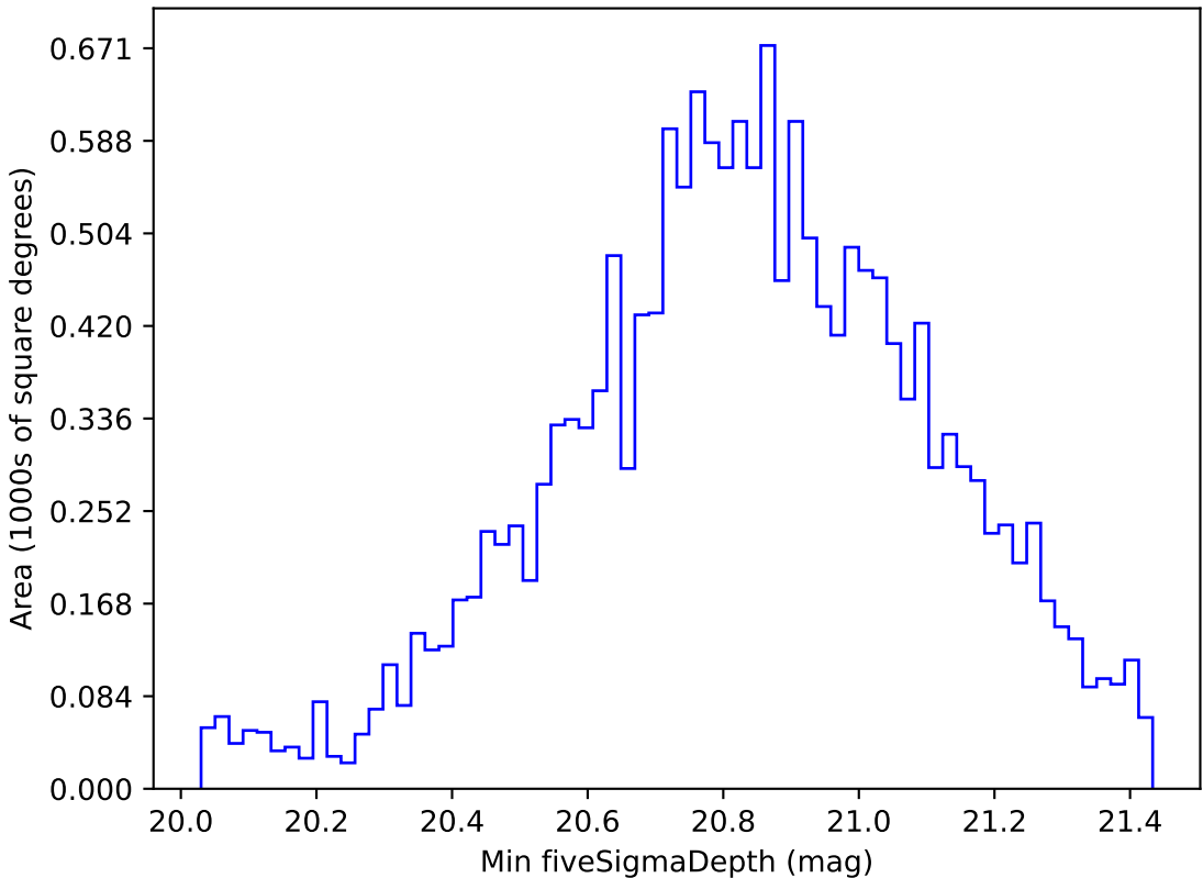
noroll_mjdp60_v3.4_10yrs WFD all bands: Min fiveSigmaDepth
