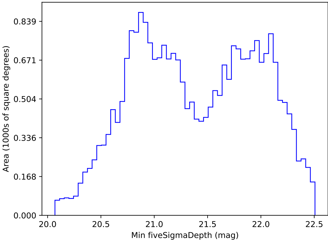
noroll_mjdp60_v3.4_10yrs All sky z band: Min fiveSigmaDepth
