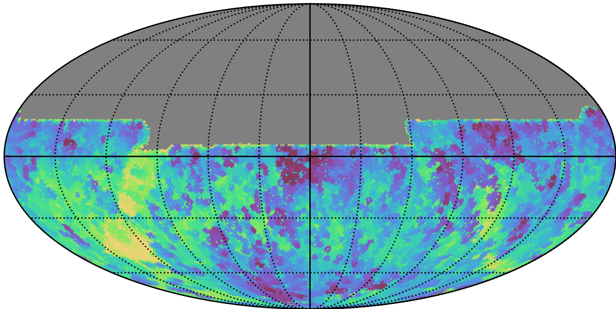
noroll_mjdp60_v3.4_10yrs All sky y band: Min fiveSigmaDepth
