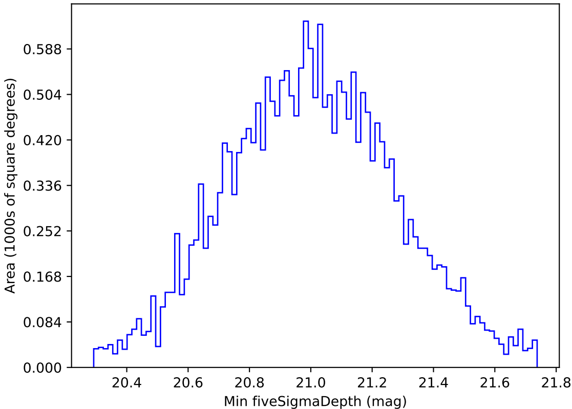
noroll_mjdp60_v3.4_10yrs All sky y band: Min fiveSigmaDepth
