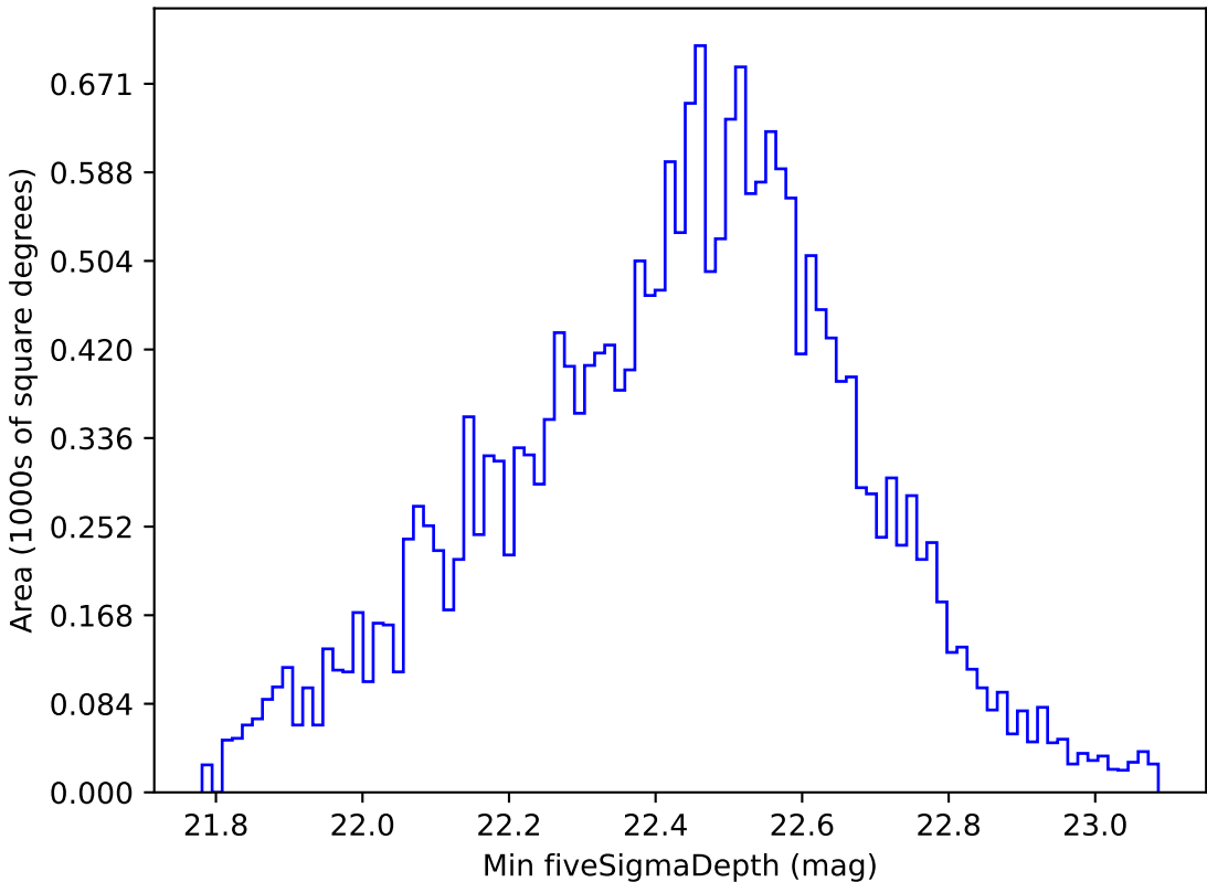
noroll_mjdp60_v3.4_10yrs All sky u band: Min fiveSigmaDepth
