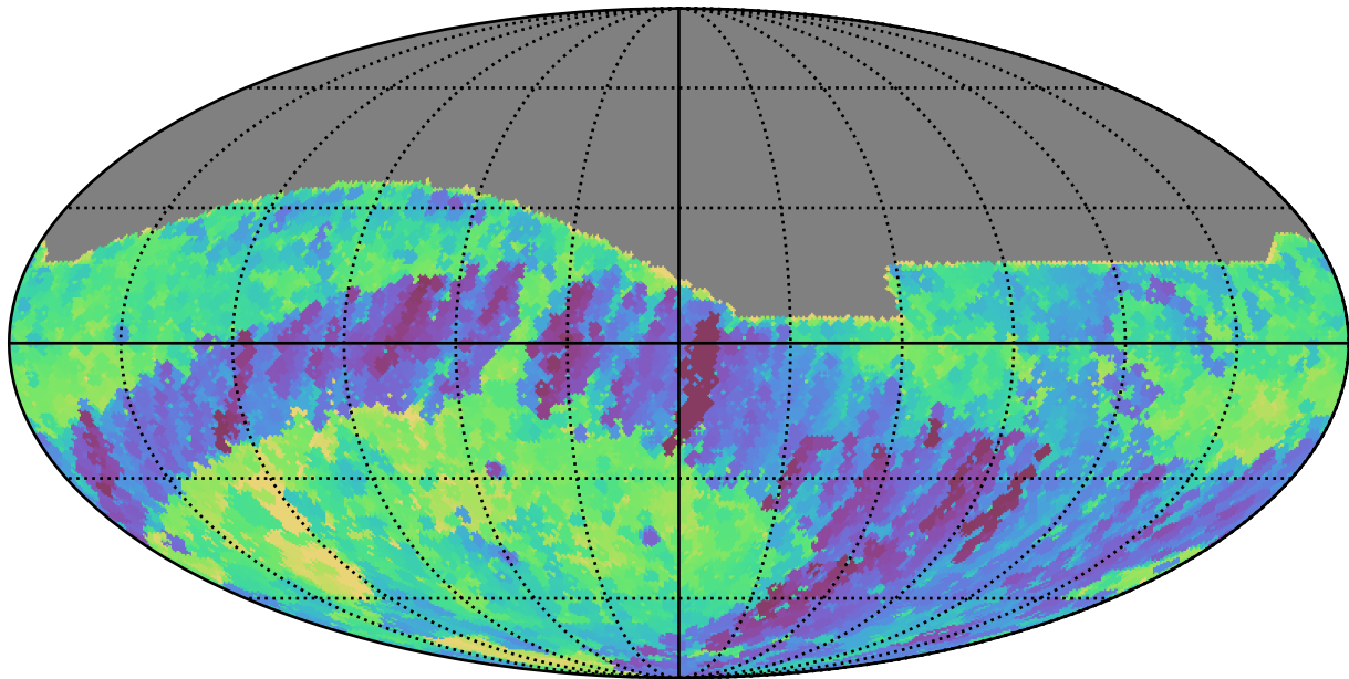
noroll_mjdp60_v3.4_10yrs All sky r band: Min fiveSigmaDepth
