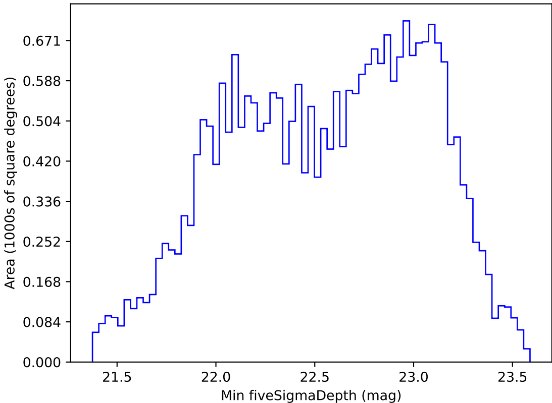
noroll_mjdp60_v3.4_10yrs All sky r band: Min fiveSigmaDepth
