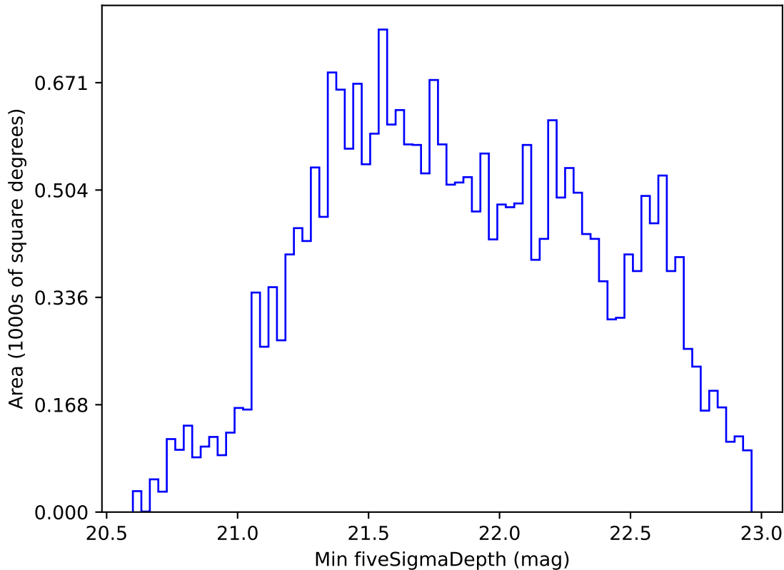
noroll_mjdp60_v3.4_10yrs All sky i band: Min fiveSigmaDepth
