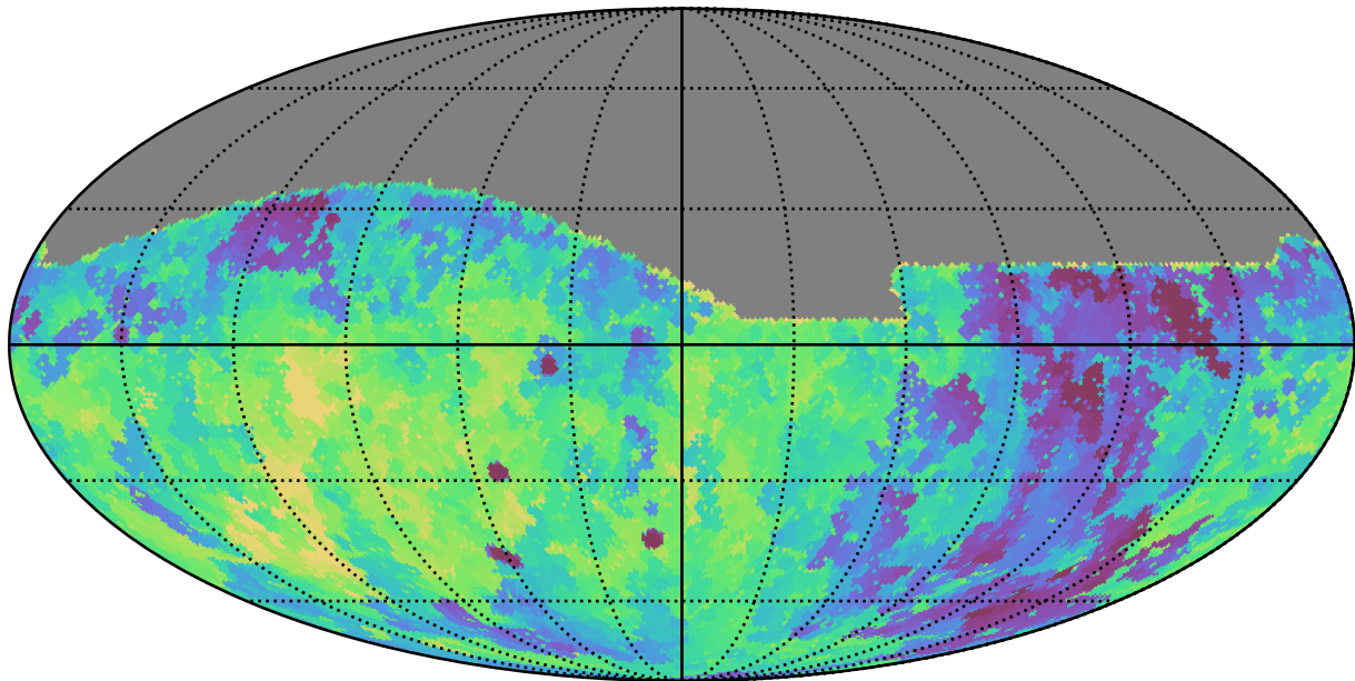
noroll_mjdp60_v3.4_10yrs All sky g band: Min fiveSigmaDepth
