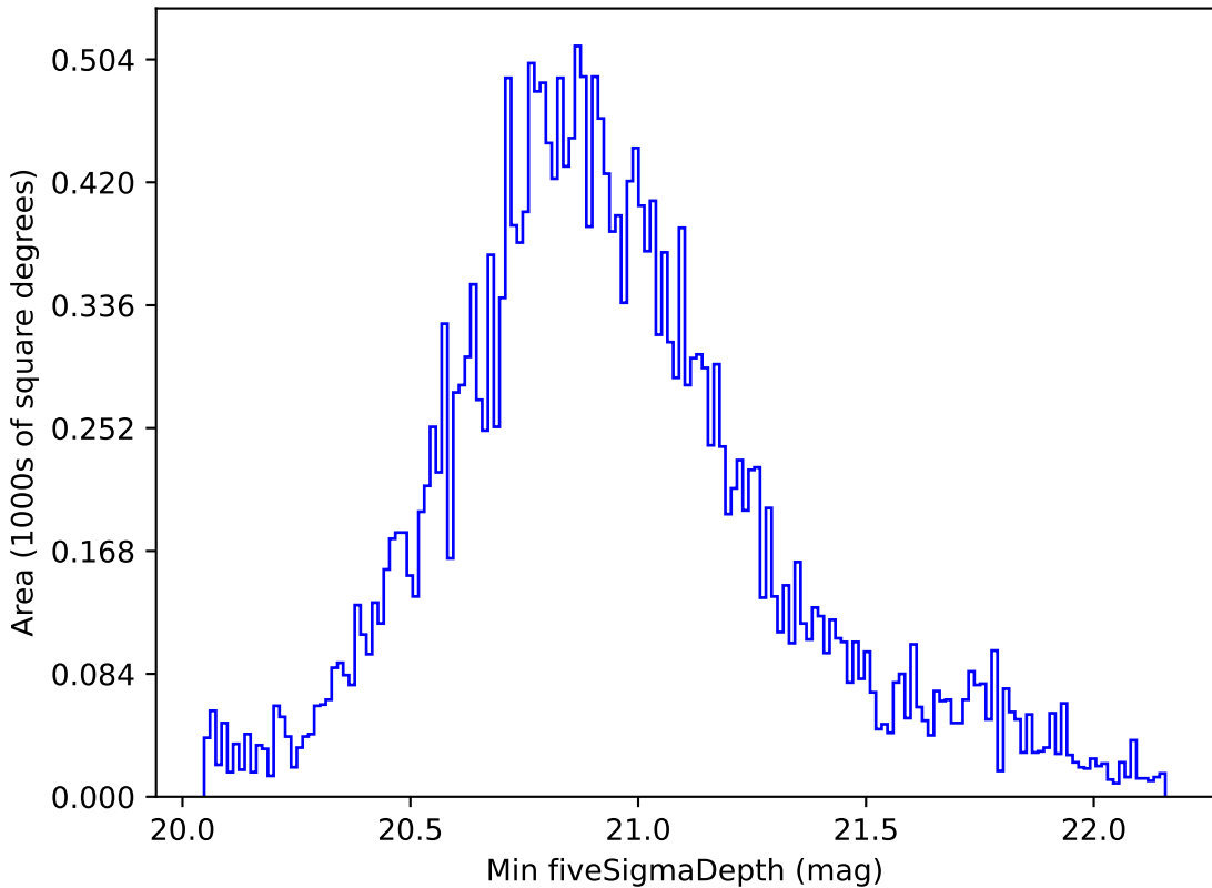
noroll_mjdp60_v3.4_10yrs All sky all bands: Min fiveSigmaDepth
