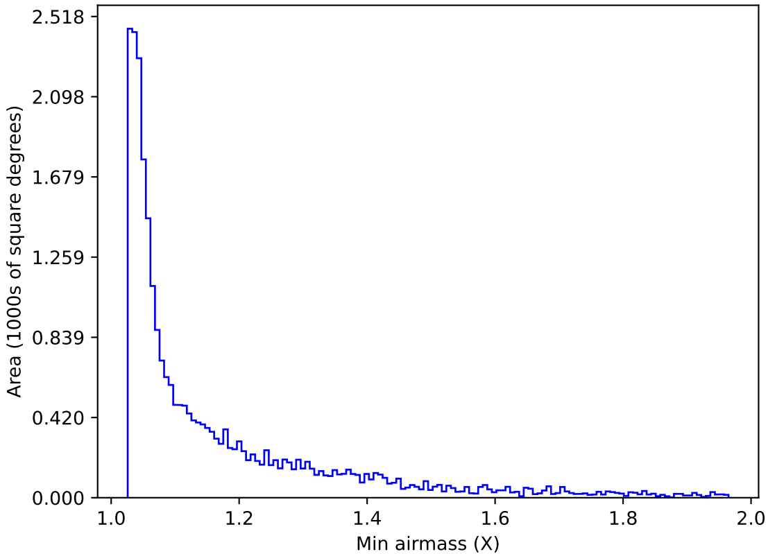
noroll_mjdp60_v3.4_10yrs Yr 1 z band: Min airmass
