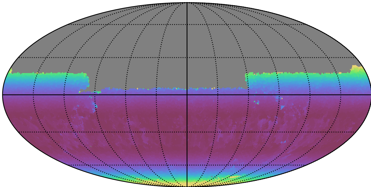
noroll_mjdp60_v3.4_10yrs Yr 1 y band: Min airmass
