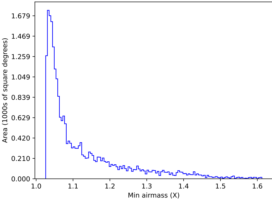
noroll_mjdp60_v3.4_10yrs Yr 1 y band: Min airmass
