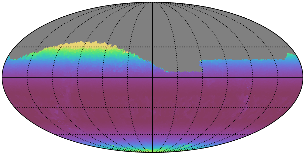
noroll_mjdp60_v3.4_10yrs Yr 1 i band: Min airmass
