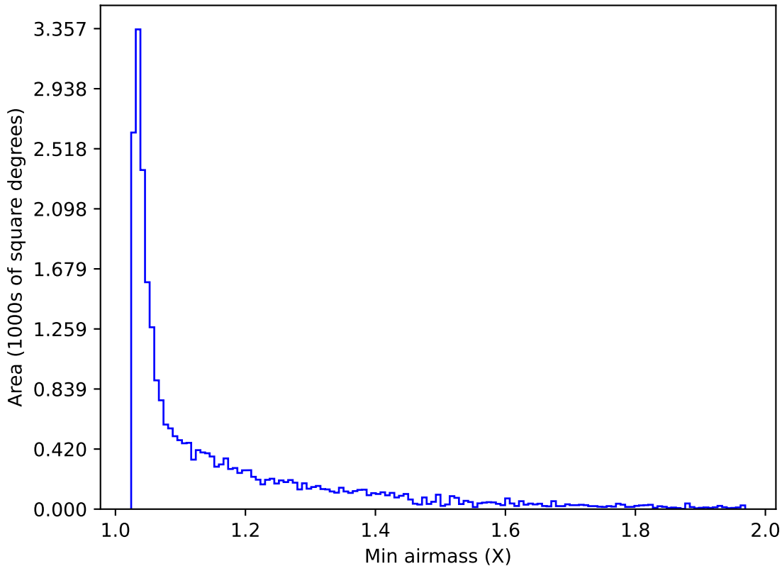
noroll_mjdp60_v3.4_10yrs Yr 1 i band: Min airmass
