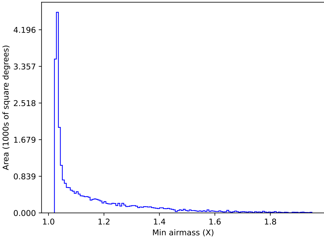
noroll_mjdp60_v3.4_10yrs Yr 1 all bands: Min airmass
