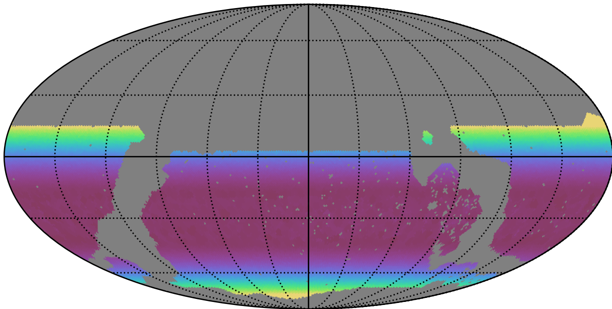
noroll_mjdp60_v3.4_10yrs WFD z band: Min airmass
