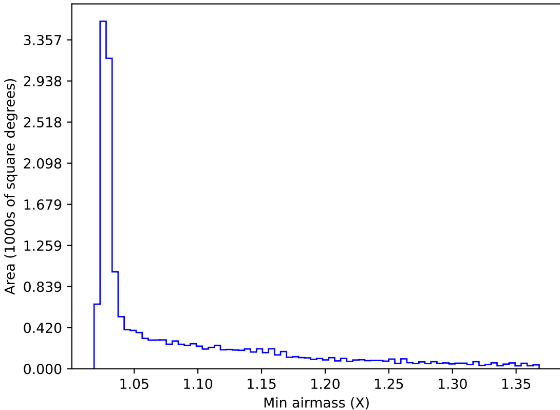
noroll_mjdp60_v3.4_10yrs WFD z band: Min airmass
