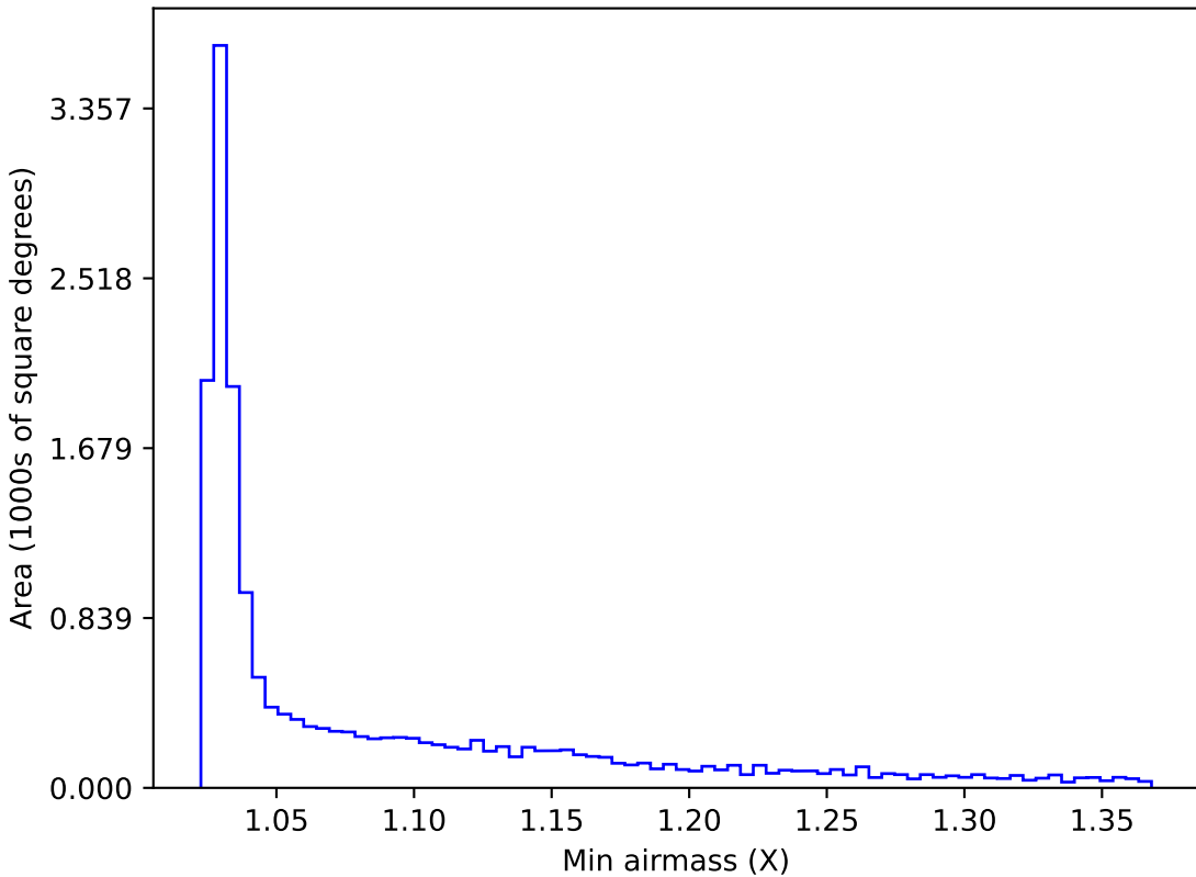
noroll_mjdp60_v3.4_10yrs WFD y band: Min airmass
