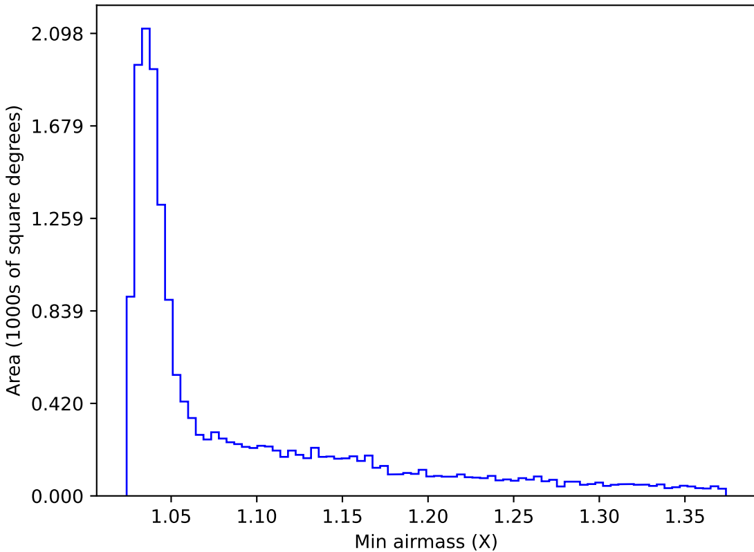
noroll_mjdp60_v3.4_10yrs WFD u band: Min airmass
