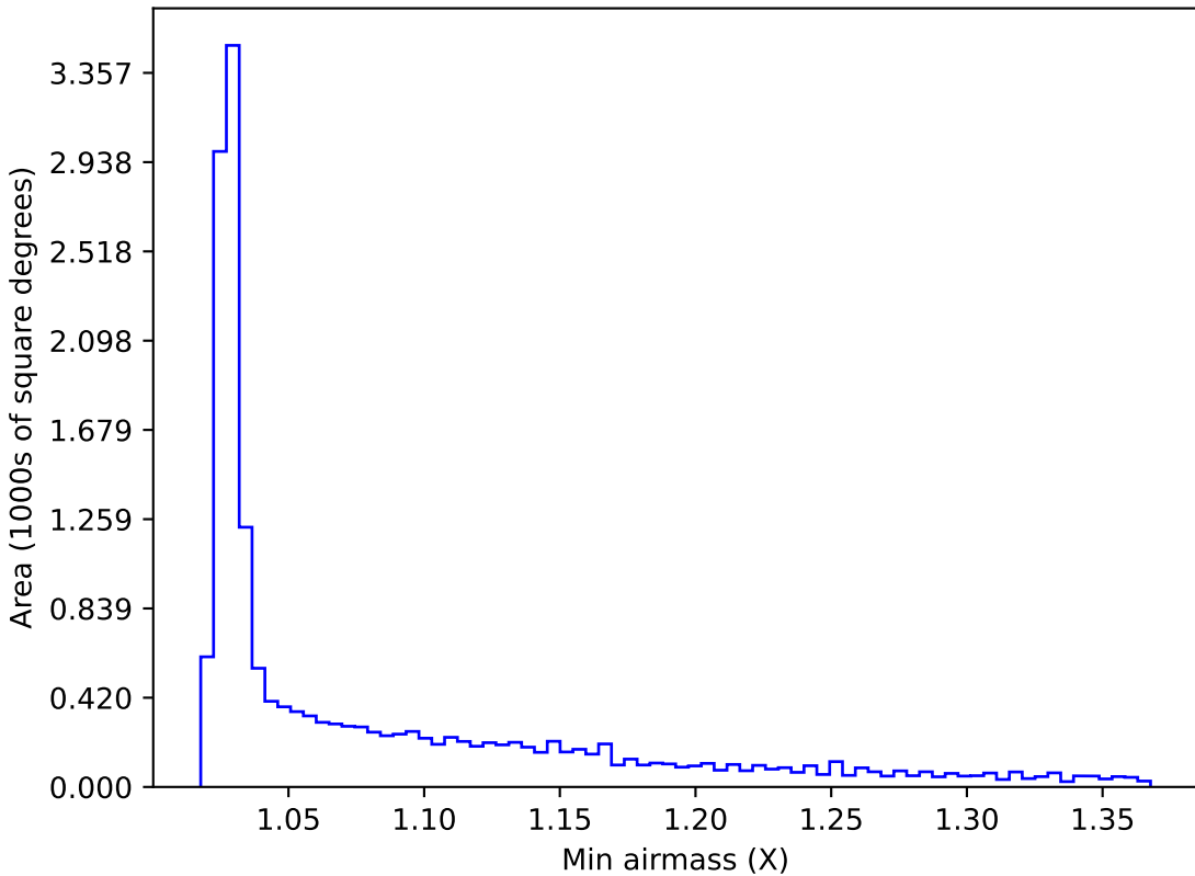
noroll_mjdp60_v3.4_10yrs WFD i band: Min airmass
