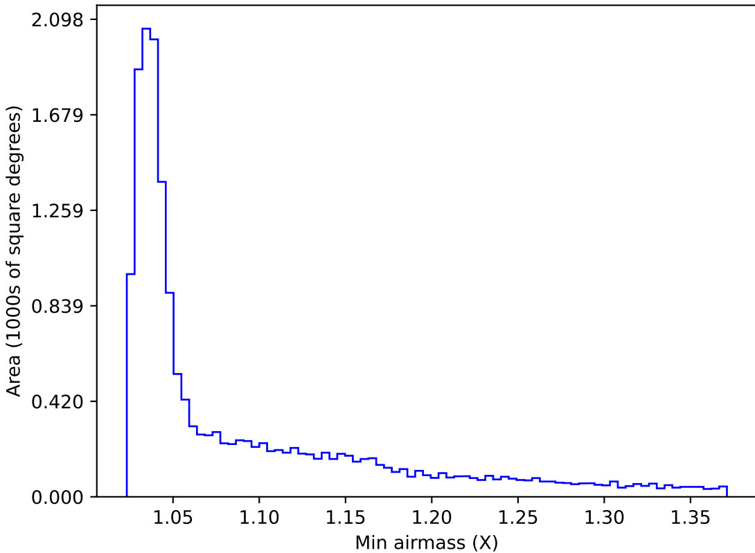
noroll_mjdp60_v3.4_10yrs WFD g band: Min airmass
