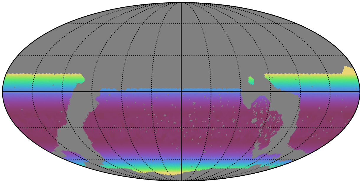
noroll_mjdp60_v3.4_10yrs WFD all bands: Min airmass
