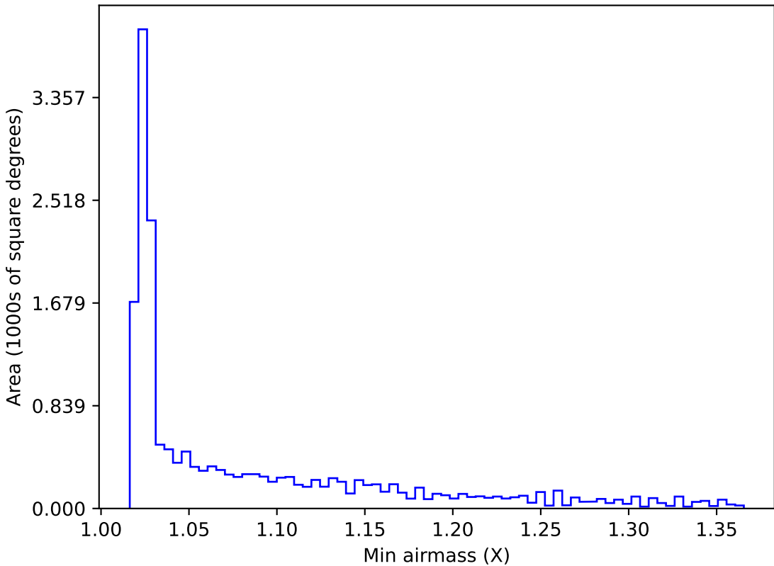
noroll_mjdp60_v3.4_10yrs WFD all bands: Min airmass
