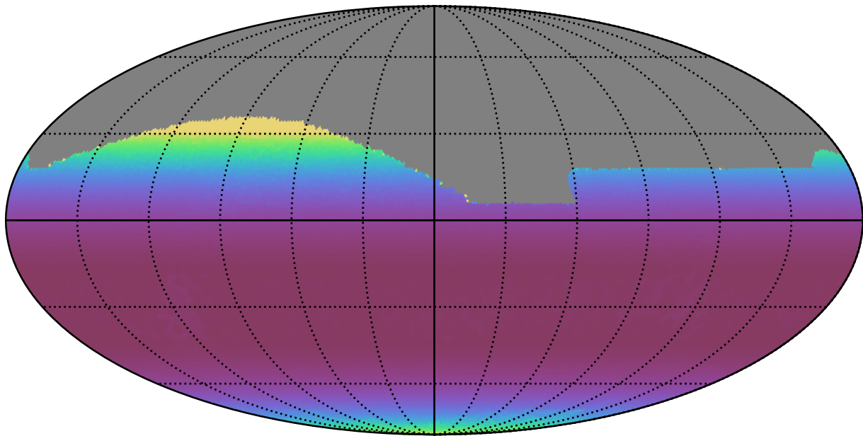
noroll_mjdp60_v3.4_10yrs All sky z band: Min airmass
