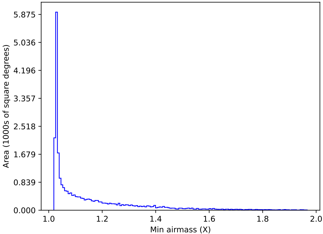
noroll_mjdp60_v3.4_10yrs All sky z band: Min airmass
