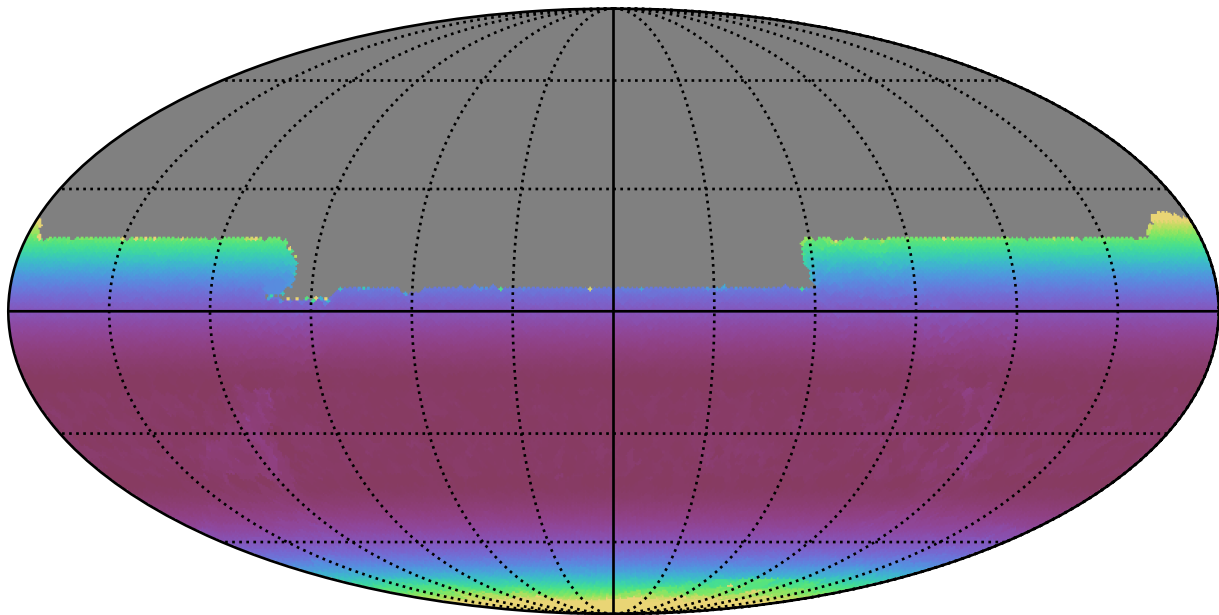
noroll_mjdp60_v3.4_10yrs All sky y band: Min airmass
