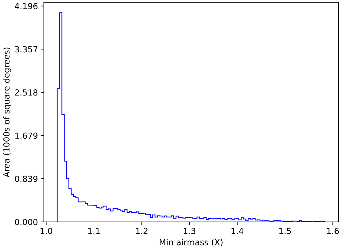
noroll_mjdp60_v3.4_10yrs All sky y band: Min airmass
