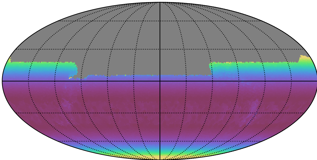
noroll_mjdp60_v3.4_10yrs All sky u band: Min airmass
