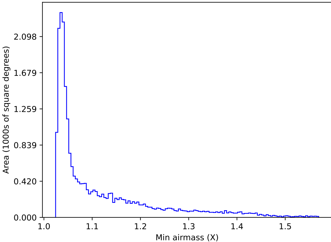
noroll_mjdp60_v3.4_10yrs All sky u band: Min airmass
