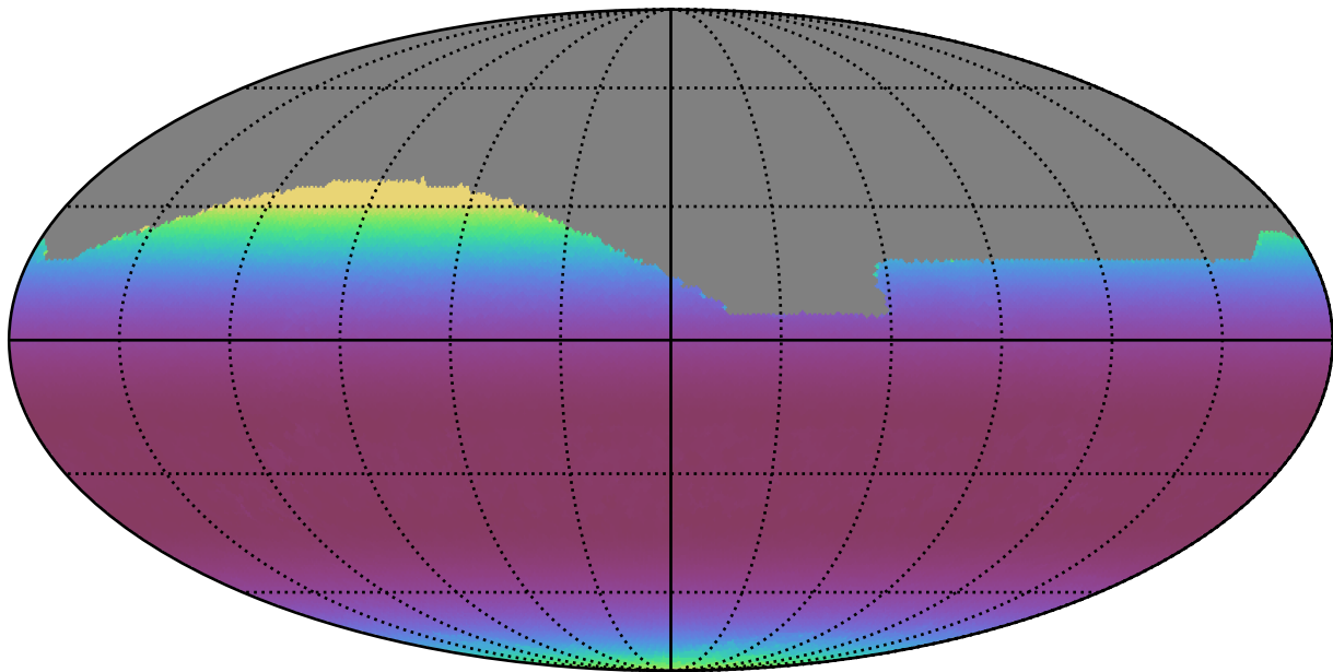
noroll_mjdp60_v3.4_10yrs All sky r band: Min airmass
