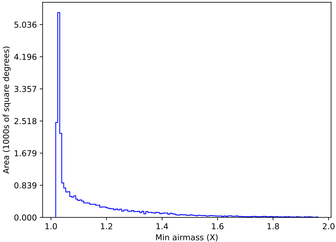
noroll_mjdp60_v3.4_10yrs All sky r band: Min airmass
